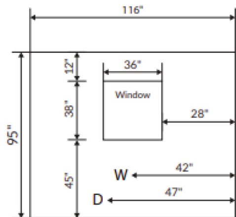
Example 2, Elevation
